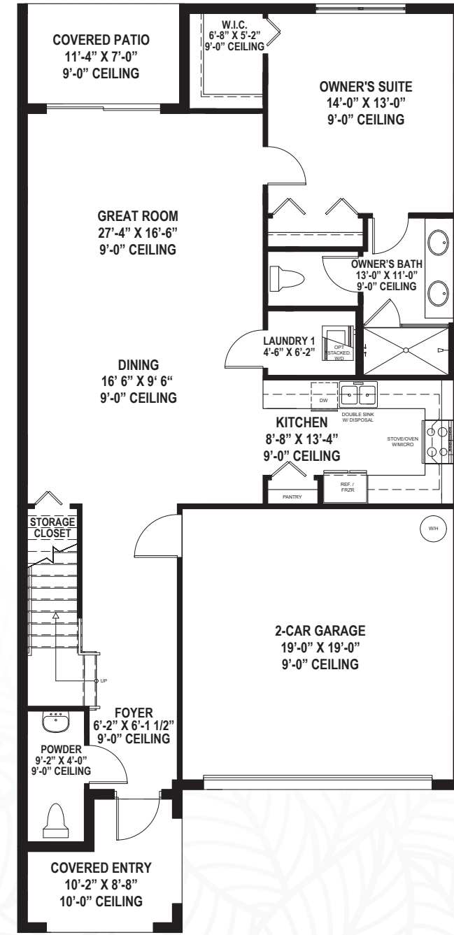
1ST FLOOR
